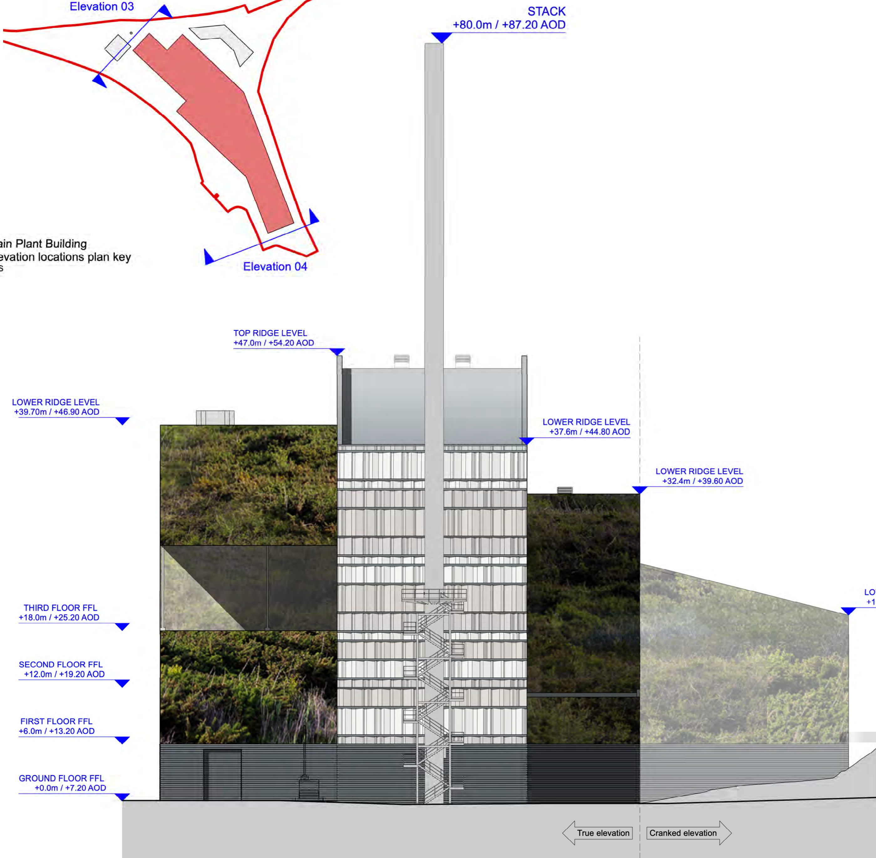
03 Elevation 03 (north-western) 1:250 @ A1 / 1:500 @ A3
